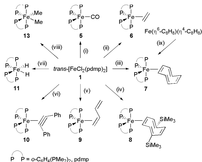
Scheme 1 (i) Na/Hg, CO; (ii) Na/Hg, \text{C}_2\text{H}_4 ; (iii) \text{K}_2\text{C}_8\text{H}_8 ; (iv) \text{Li}_2\{1,4\text{-C}_8\text{H}_6(\text{SiMe}_3)_2\} ; (v) \text{C}_4\text{H}_6\text{Mg}\cdot 2\text{thf} ; (vi) \text{NaC}_{10}\text{H}_8 , \text{PhC}_2\text{Ph} ; (vii) Na/Hg, \text{H}_2 or \text{LiAlH}_4 ; (viii) MeLi (excess); (ix) pdmp.
